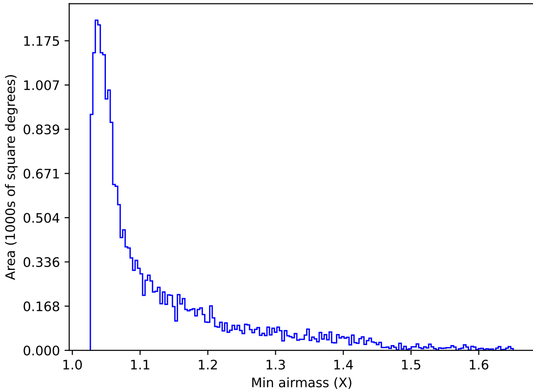
weather_cloudso30v3.4_10yrs Yr 1 y band: Min airmass
