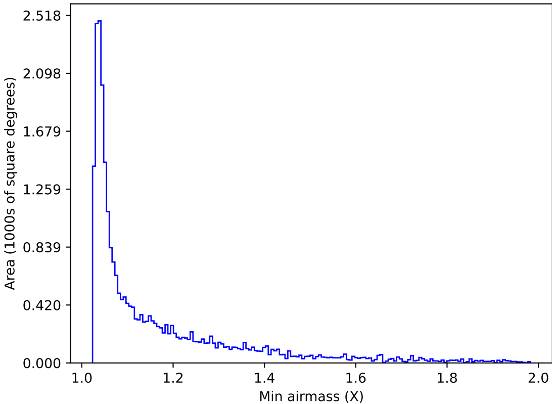
weather_cloudso30v3.4_10yrs Yr 1 r band: Min airmass
