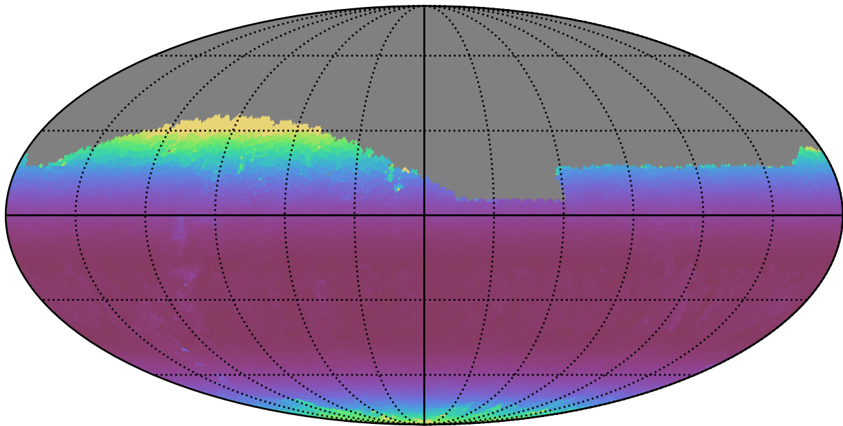
weather_cloudso30v3.4_10yrs Yr 1 i band: Min airmass
