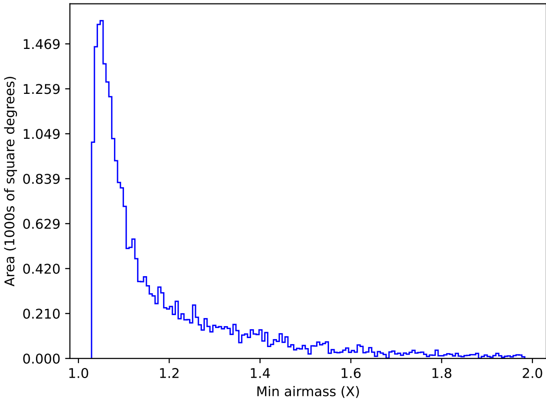
weather_cloudso30v3.4_10yrs Yr 1 g band: Min airmass
