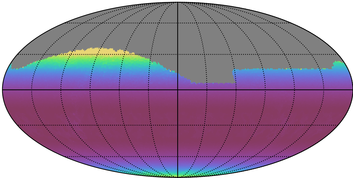
weather_cloudso30v3.4_10yrs Yr 1 all bands: Min airmass
