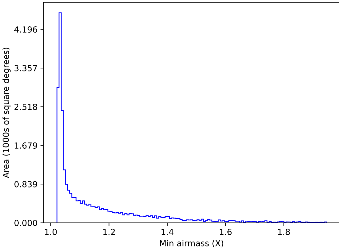
weather_cloudso30v3.4_10yrs Yr 1 all bands: Min airmass
