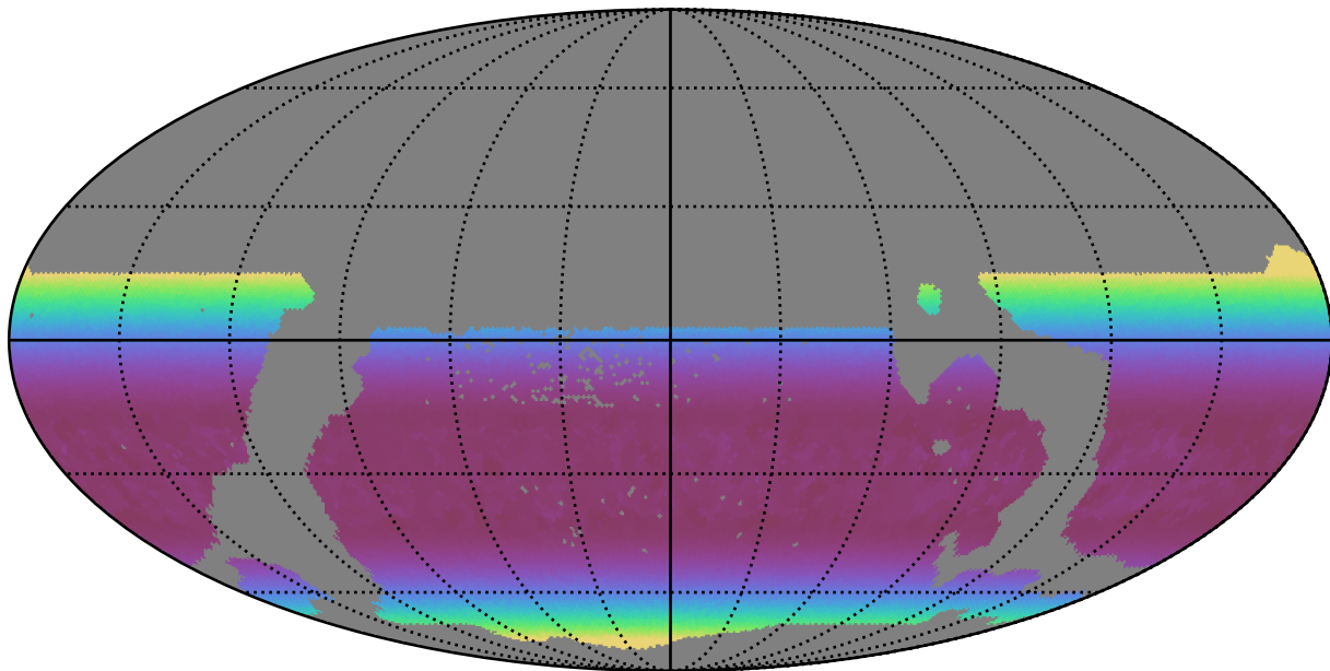
weather_cloudso30v3.4_10yrs WFD z band: Min airmass
