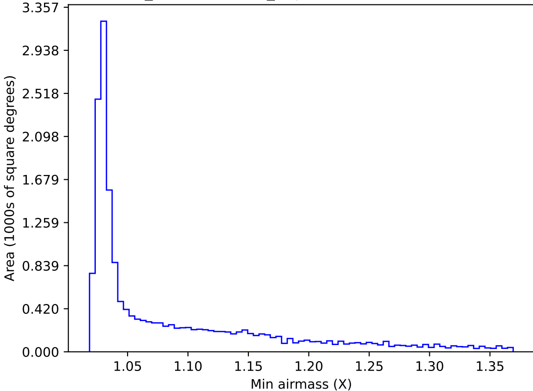
weather_cloudso30v3.4_10yrs WFD z band: Min airmass
