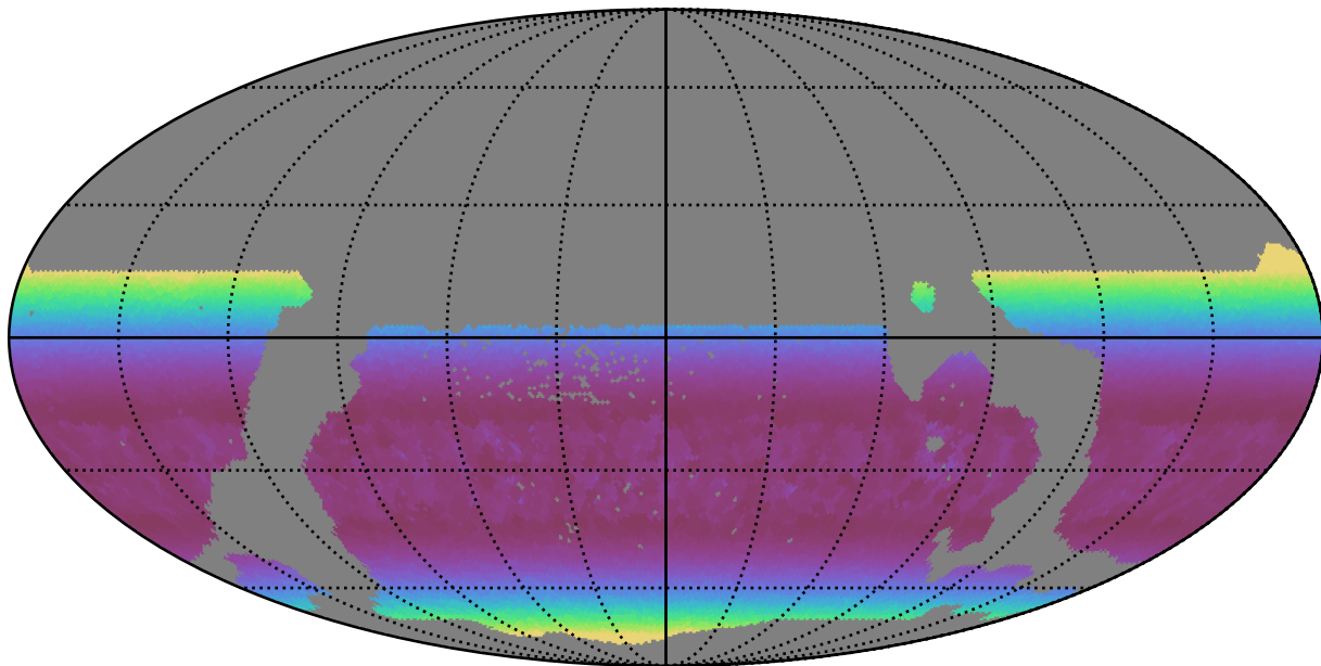
weather_cloudso30v3.4_10yrs WFD u band: Min airmass
