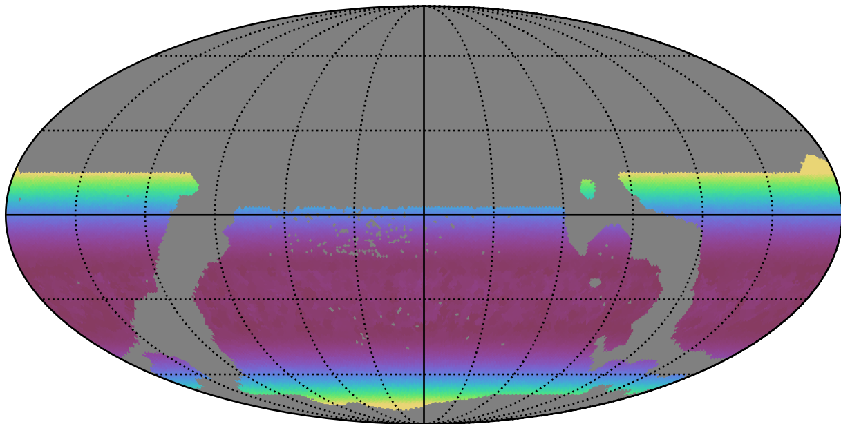
weather_cloudso30v3.4_10yrs WFD r band: Min airmass
