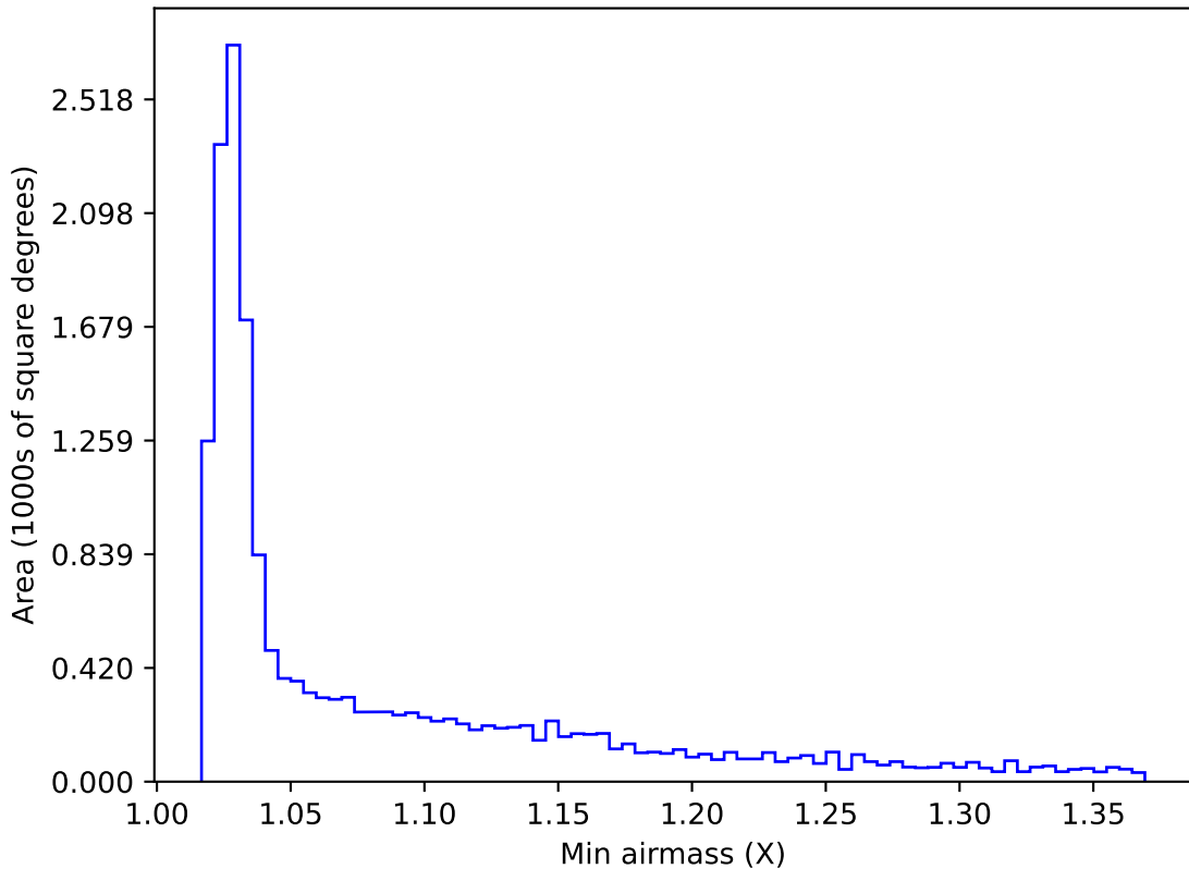
weather_cloudso30v3.4_10yrs WFD r band: Min airmass
