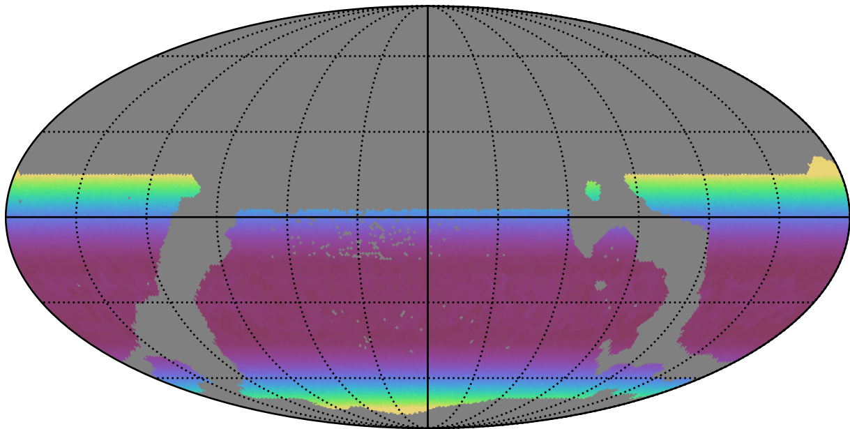
weather_cloudso30v3.4_10yrs WFD i band: Min airmass
