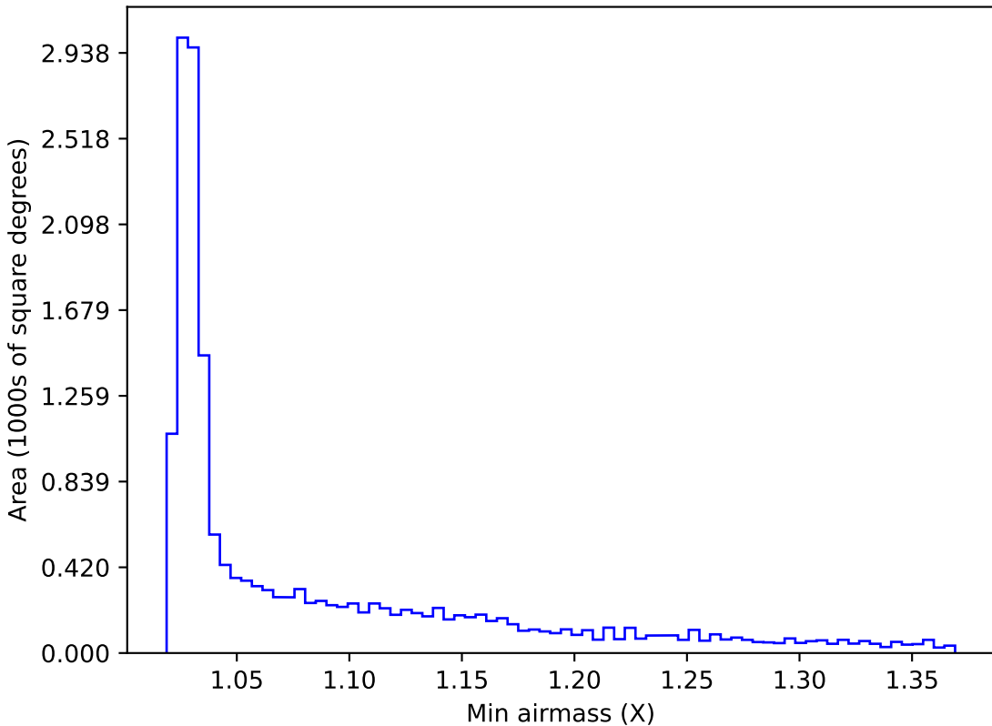
weather_cloudso30v3.4_10yrs WFD i band: Min airmass
