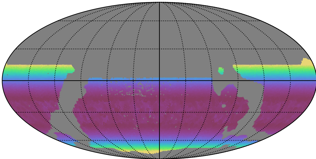
weather_cloudso30v3.4_10yrs WFD g band: Min airmass
