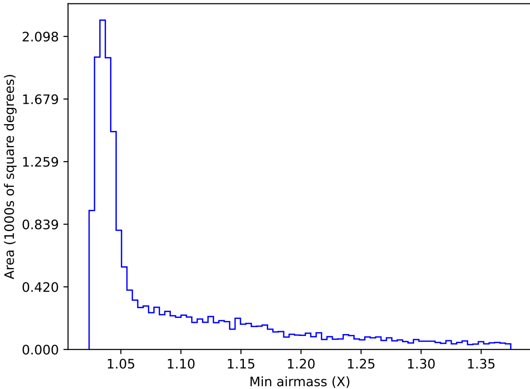
weather_cloudso30v3.4_10yrs WFD g band: Min airmass
