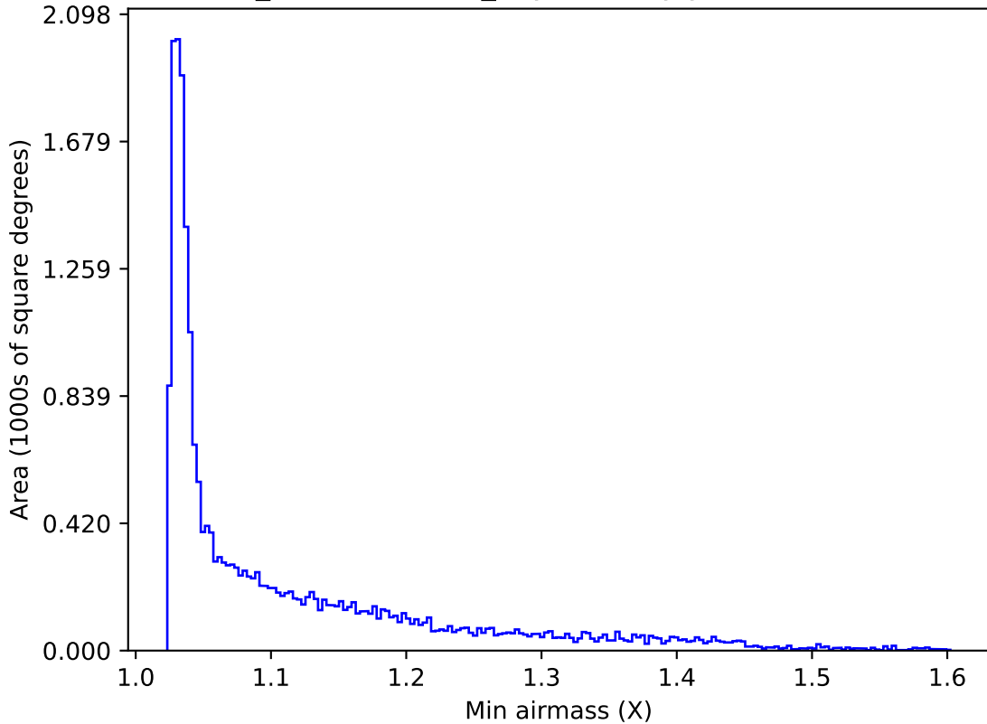
weather_cloudso30v3.4_10yrs All sky y band: Min airmass
