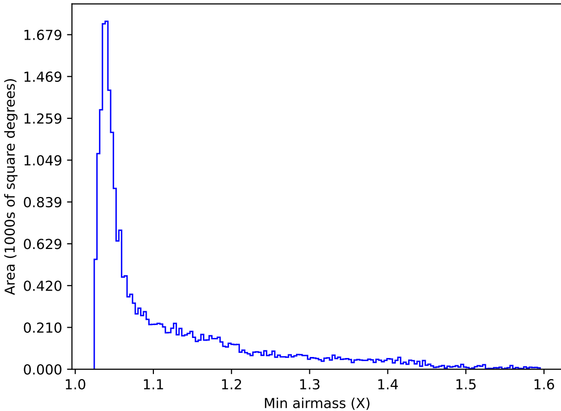
weather_cloudso30v3.4_10yrs All sky u band: Min airmass
