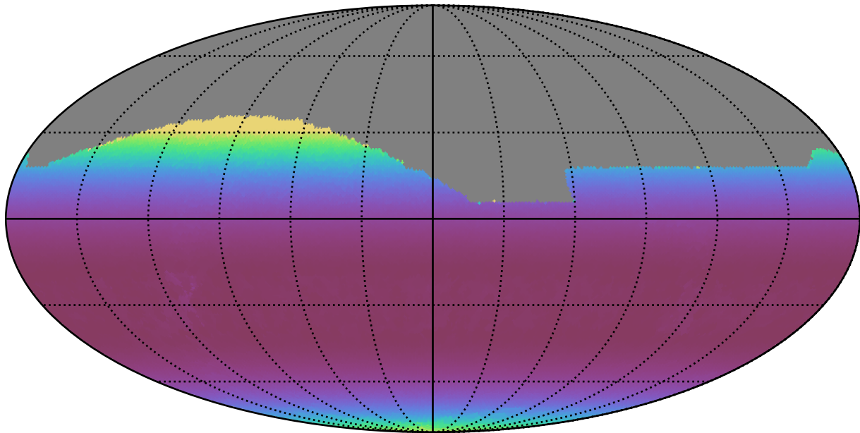
weather_cloudso30v3.4_10yrs All sky r band: Min airmass
