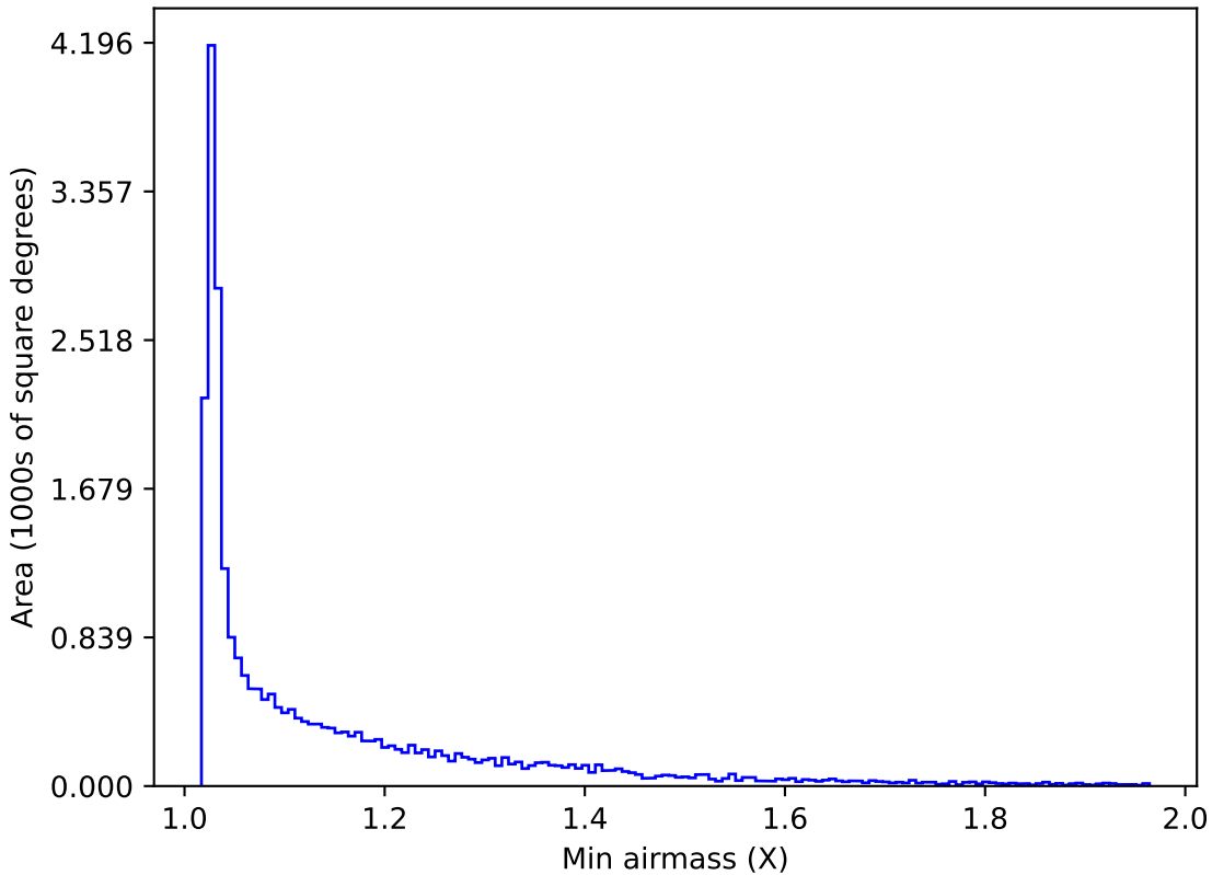
weather_cloudso30v3.4_10yrs All sky r band: Min airmass
