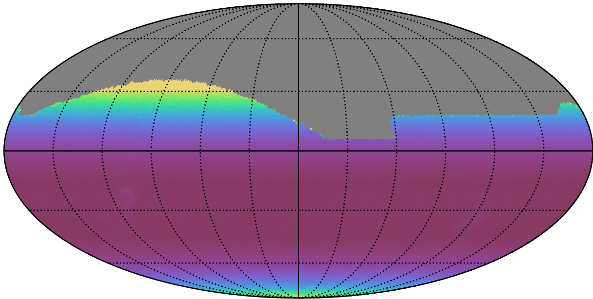
weather_cloudso30v3.4_10yrs All sky i band: Min airmass
