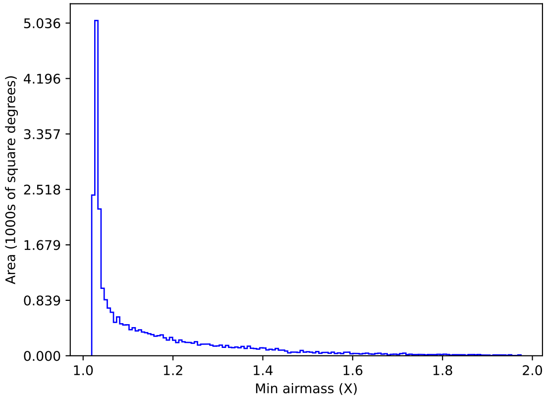
weather_cloudso30v3.4_10yrs All sky i band: Min airmass
