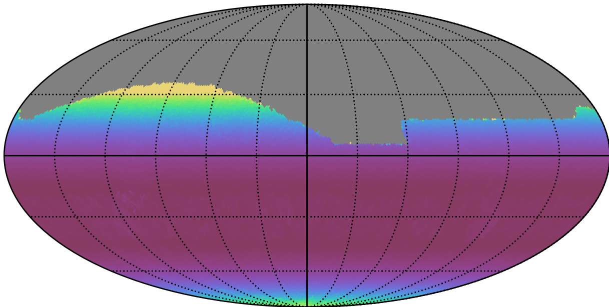
weather_cloudso30v3.4_10yrs All sky g band: Min airmass
