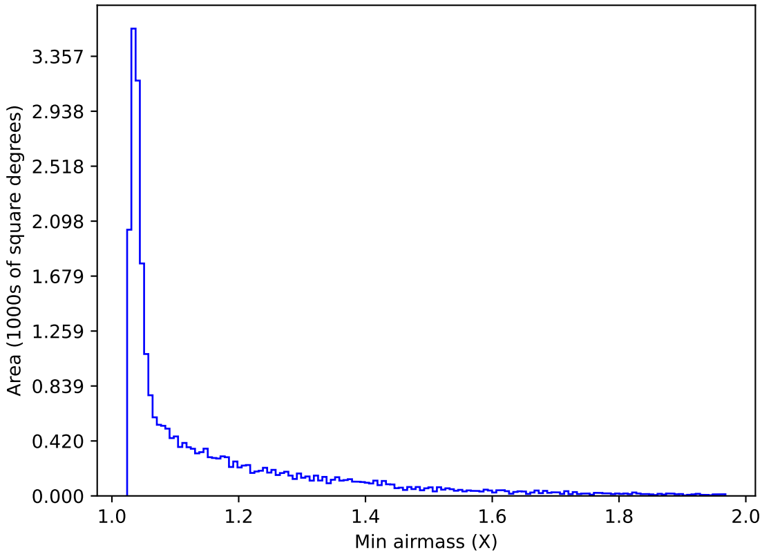
weather_cloudso30v3.4_10yrs All sky g band: Min airmass
