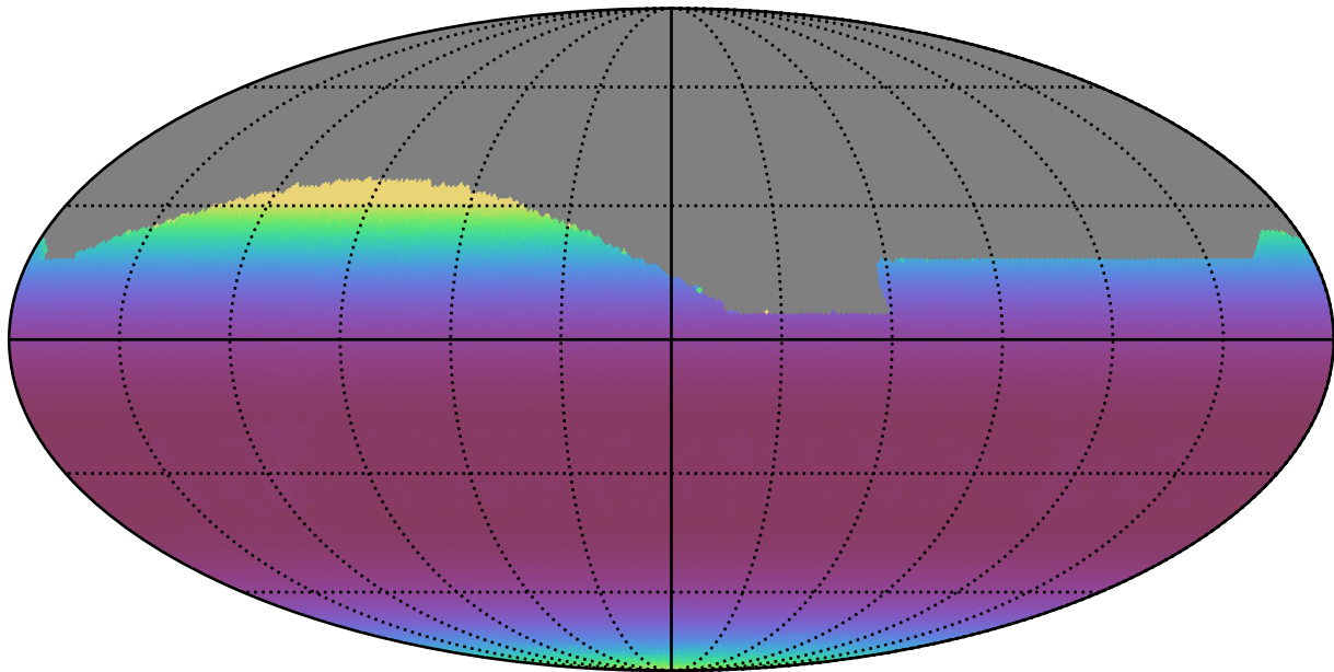
weather_cloudso30v3.4_10yrs All sky all bands: Min airmass
