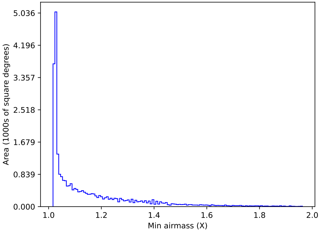
weather_cloudso30v3.4_10yrs All sky all bands: Min airmass
