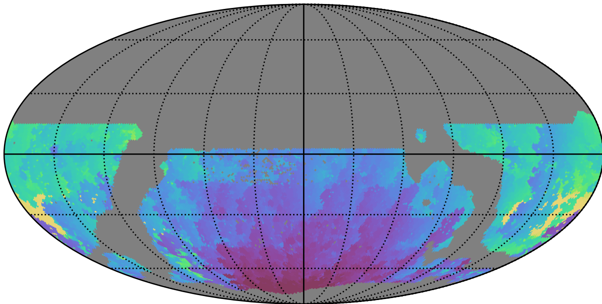
weather_cloudso30v3.4_10yrs WFD u band: Min HA
