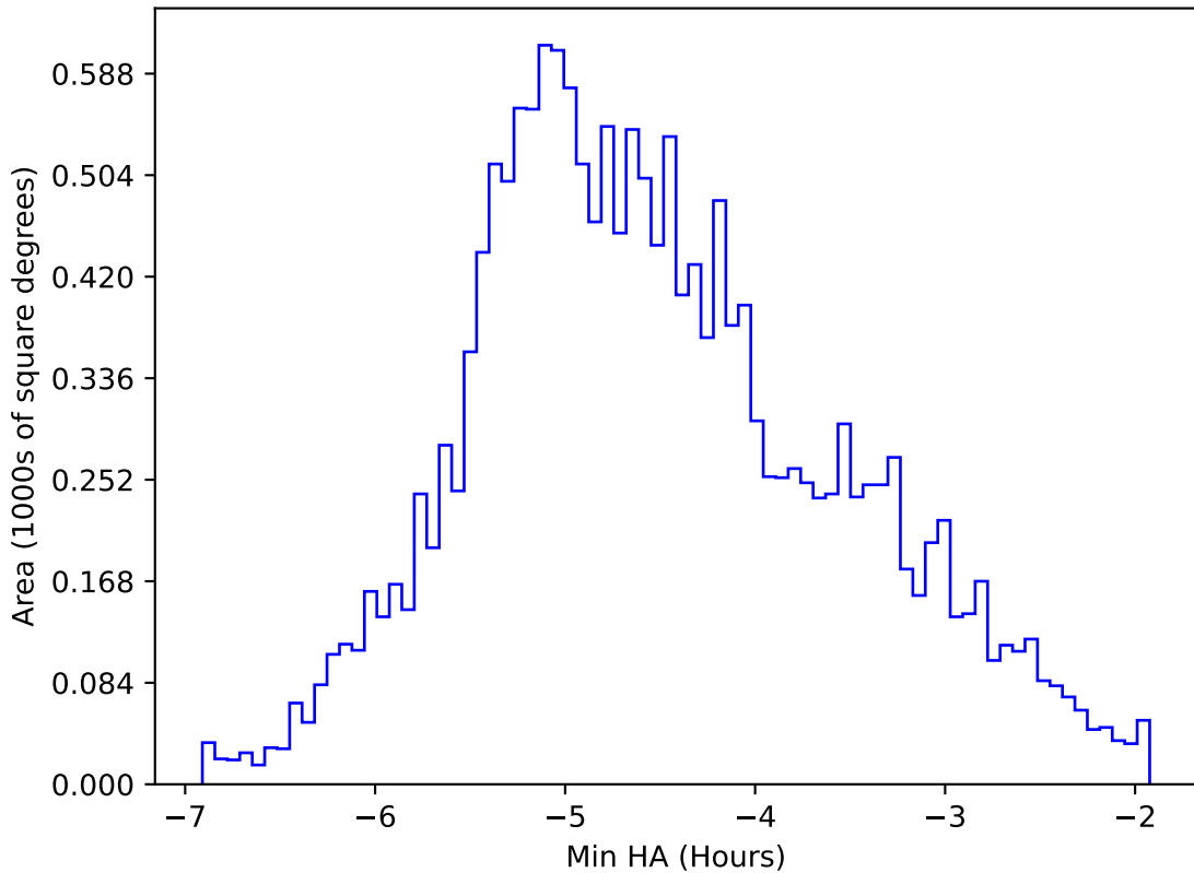
weather_cloudso30v3.4_10yrs WFD r band: Min HA
