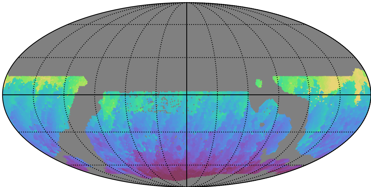
weather_cloudso30v3.4_10yrs WFD g band: Min HA
