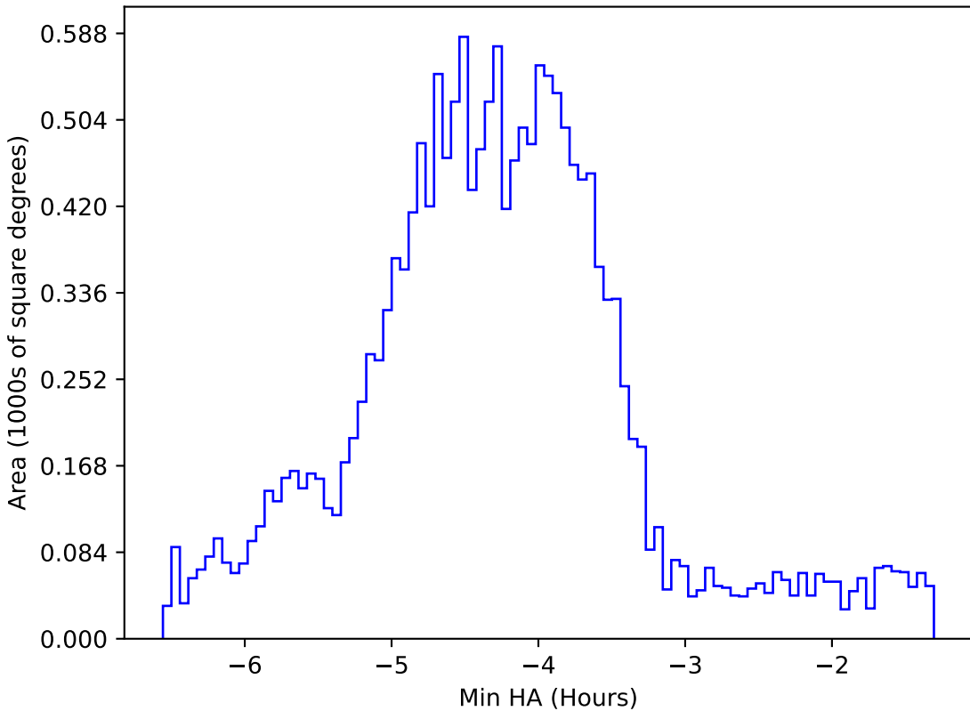
weather_cloudso30v3.4_10yrs WFD g band: Min HA
