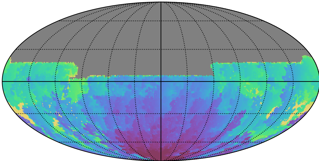
weather_cloudso30v3.4_10yrs All sky u band: Min HA
