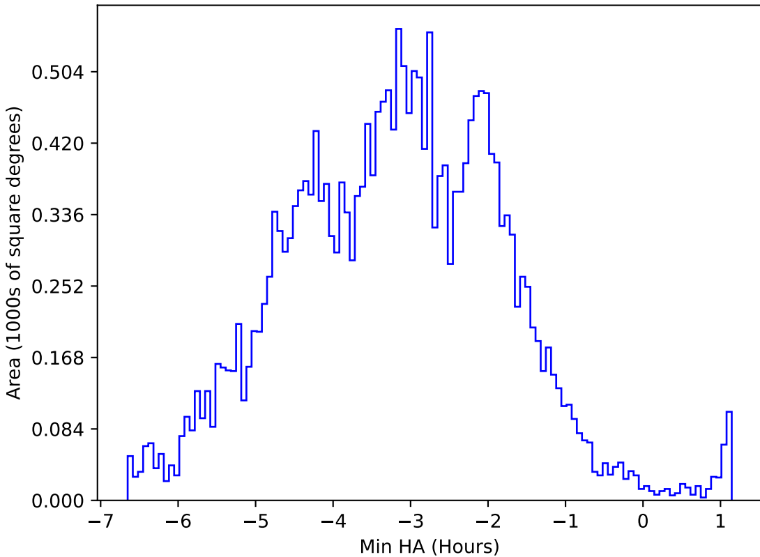
weather_cloudso30v3.4_10yrs All sky u band: Min HA
