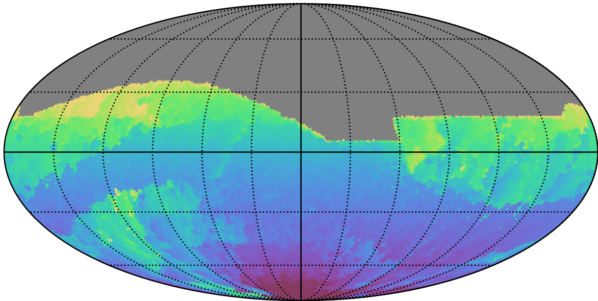
weather_cloudso30v3.4_10yrs All sky r band: Min HA
