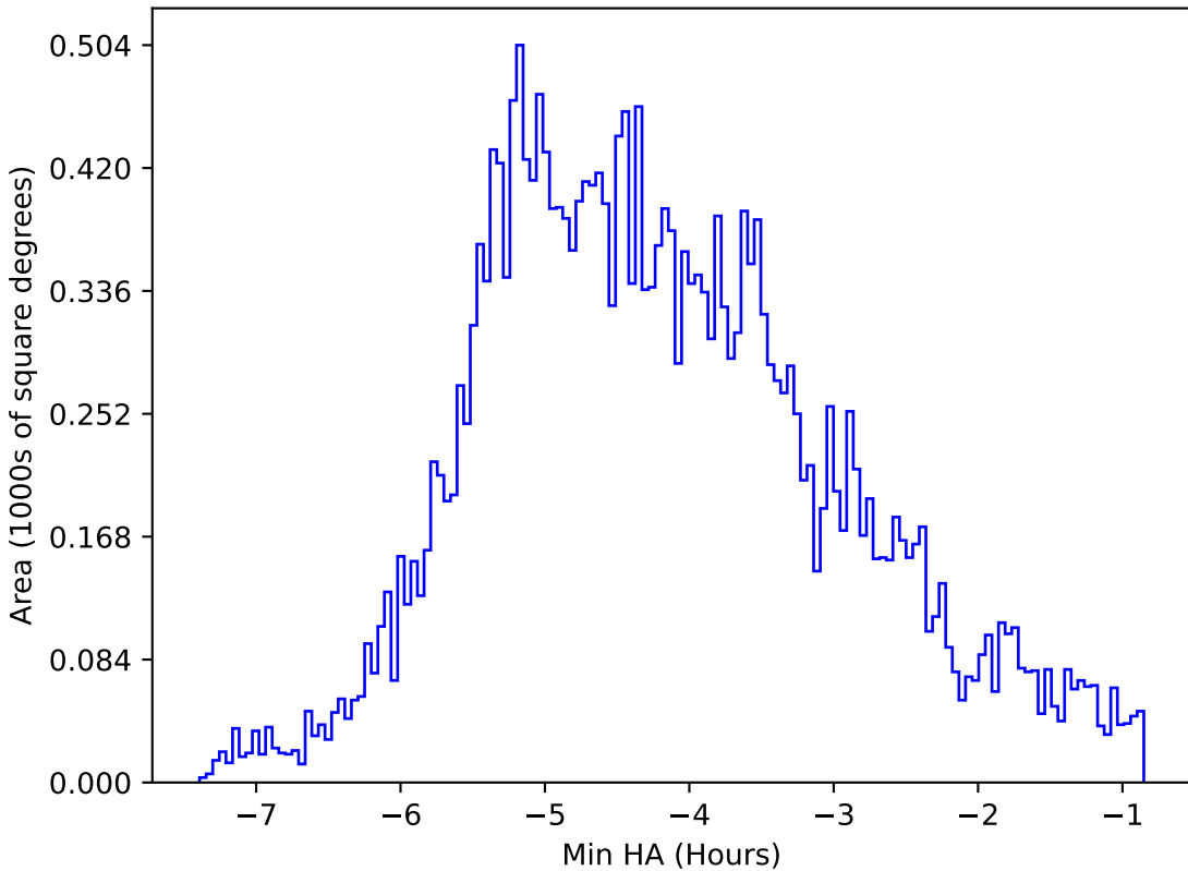
weather_cloudso30v3.4_10yrs All sky r band: Min HA
