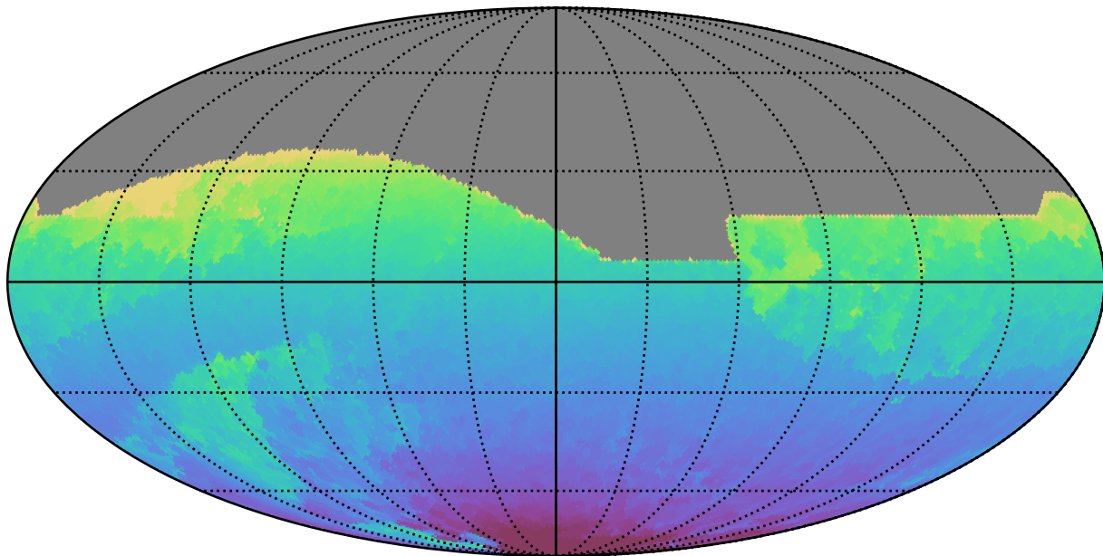
weather_cloudso30v3.4_10yrs All sky all bands: Min HA
