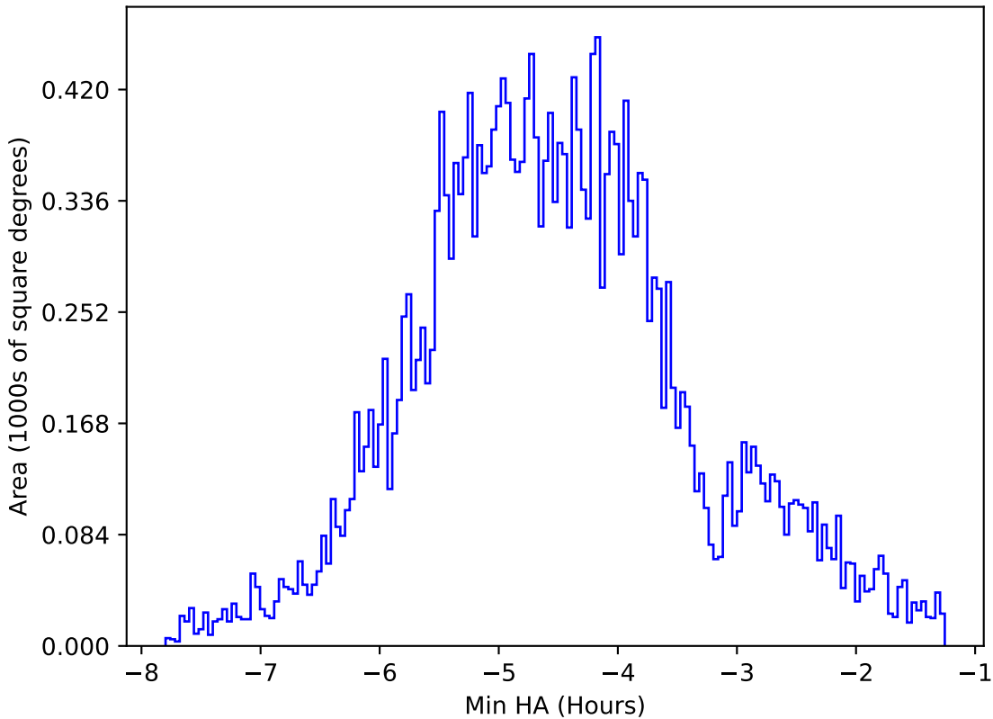
weather_cloudso30v3.4_10yrs All sky all bands: Min HA
