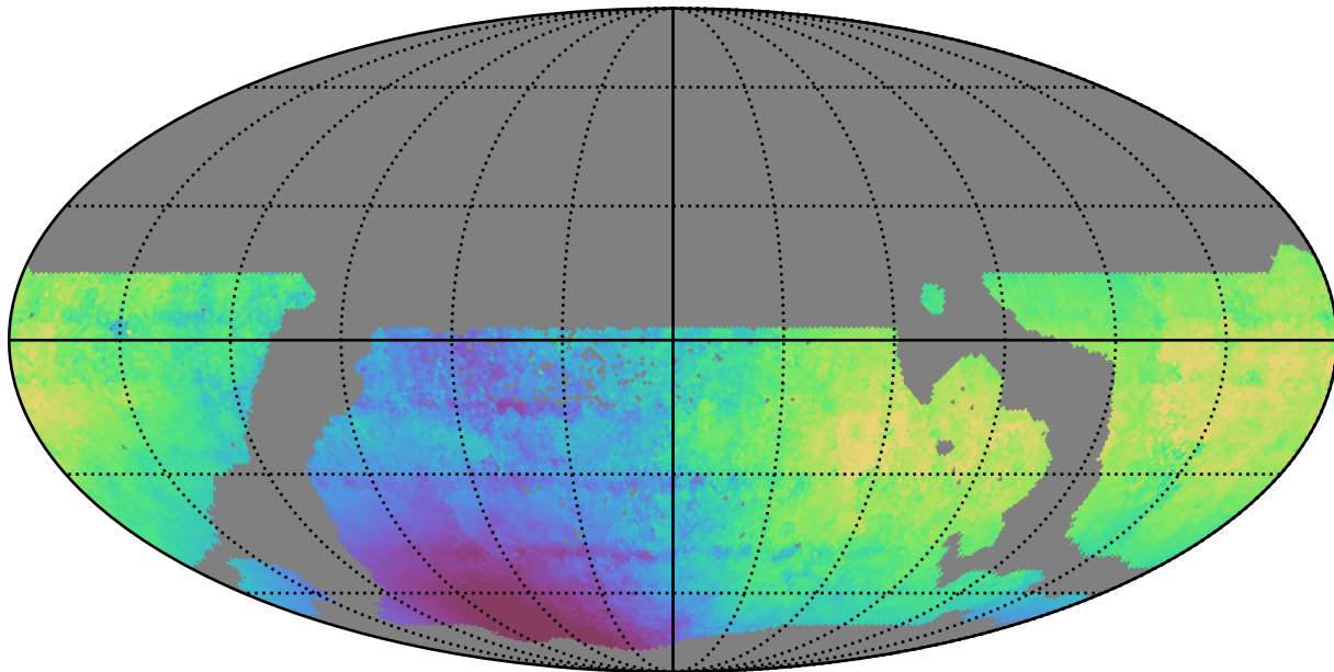
weather_cloudso30v3.4_10yrs WFD z band: Median solarElong
