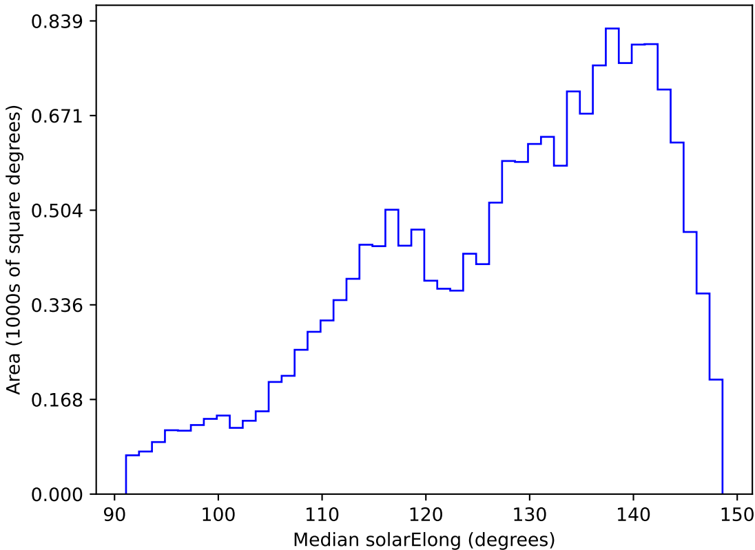
weather_cloudso30v3.4_10yrs WFD z band: Median solarElong
