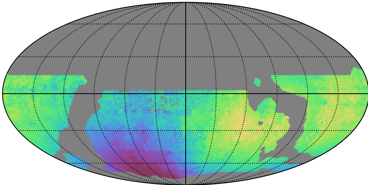
weather_cloudso30v3.4_10yrs WFD y band: Median solarElong
