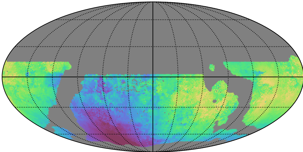
weather_cloudso30v3.4_10yrs WFD u band: Median solarElong
