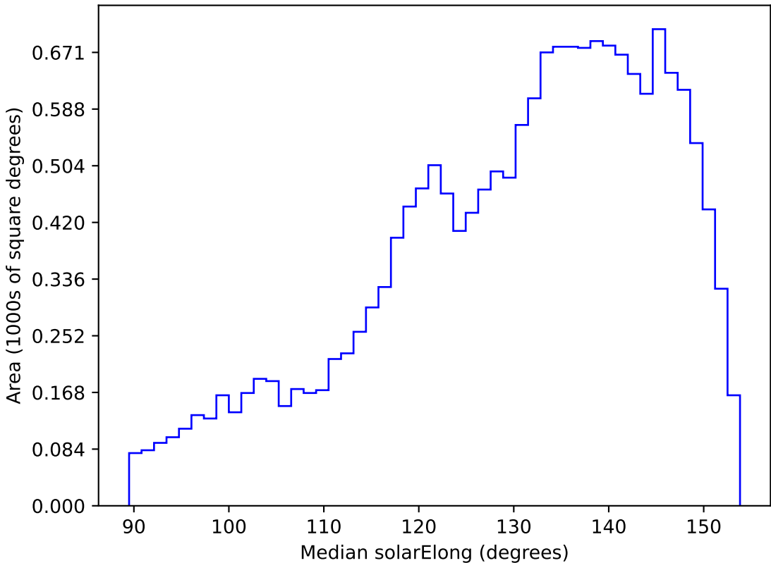
weather_cloudso30v3.4_10yrs WFD u band: Median solarElong
