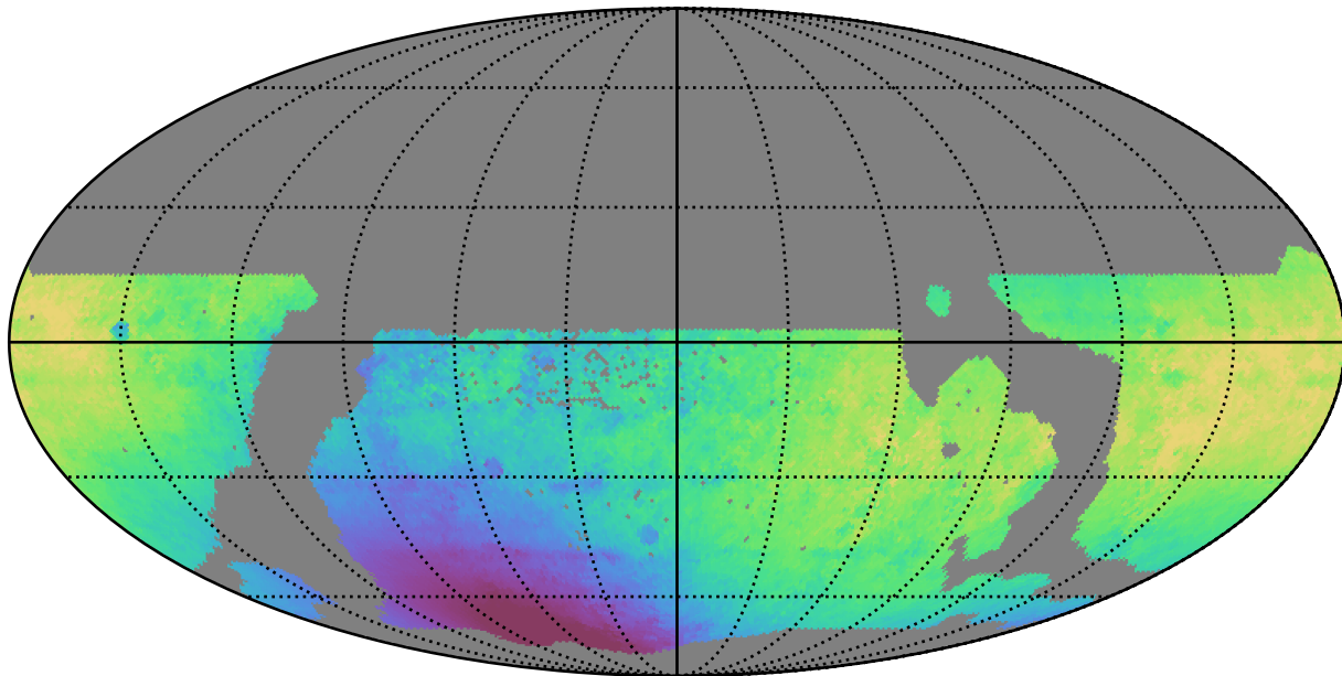
weather_cloudso30v3.4_10yrs WFD r band: Median solarElong
