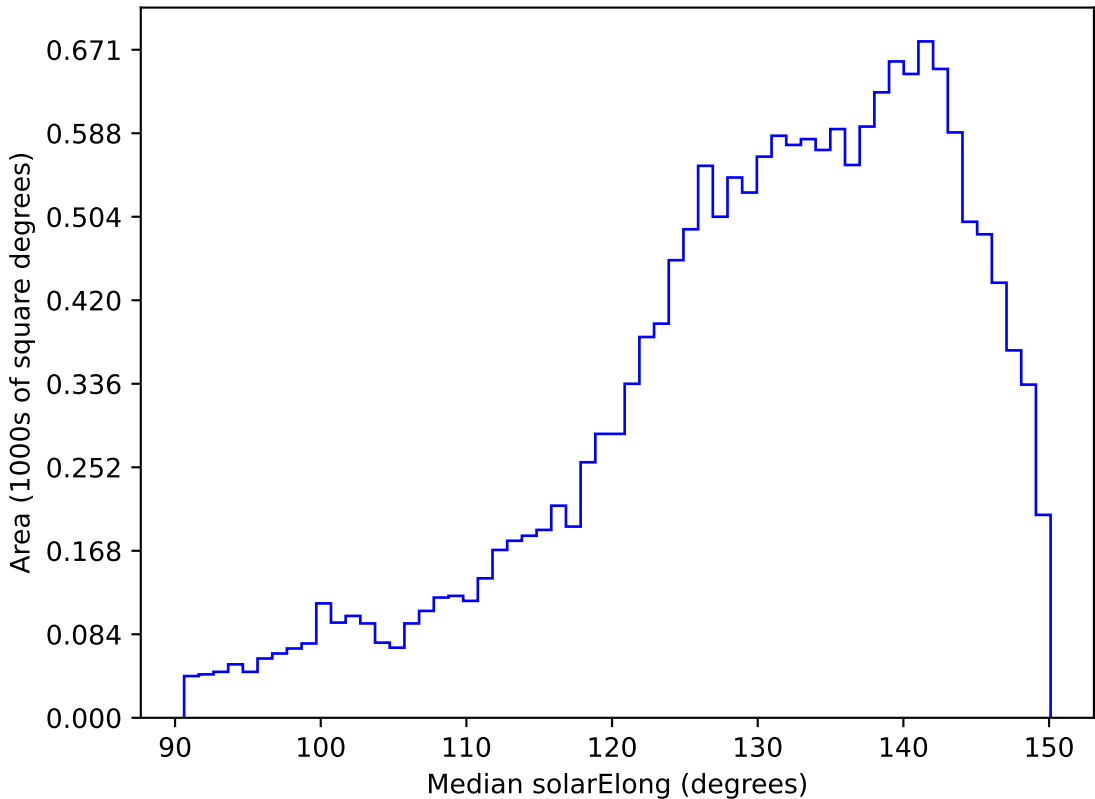
weather_cloudso30v3.4_10yrs WFD r band: Median solarElong
