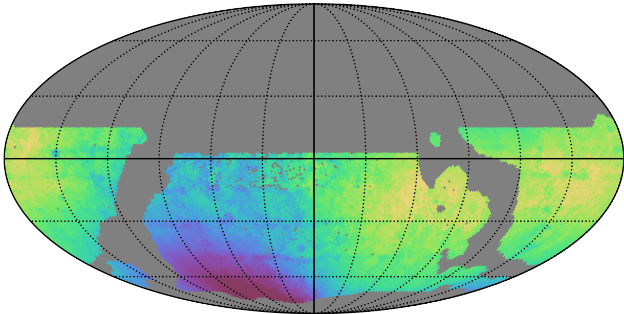
weather_cloudso30v3.4_10yrs WFD i band: Median solarElong
