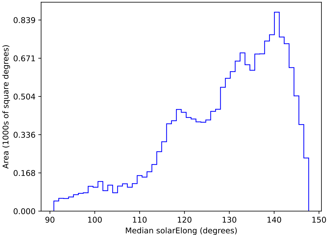
weather_cloudso30v3.4_10yrs WFD i band: Median solarElong
