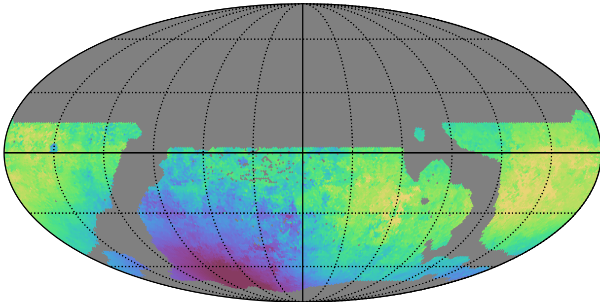
weather_cloudso30v3.4_10yrs WFD g band: Median solarElong
