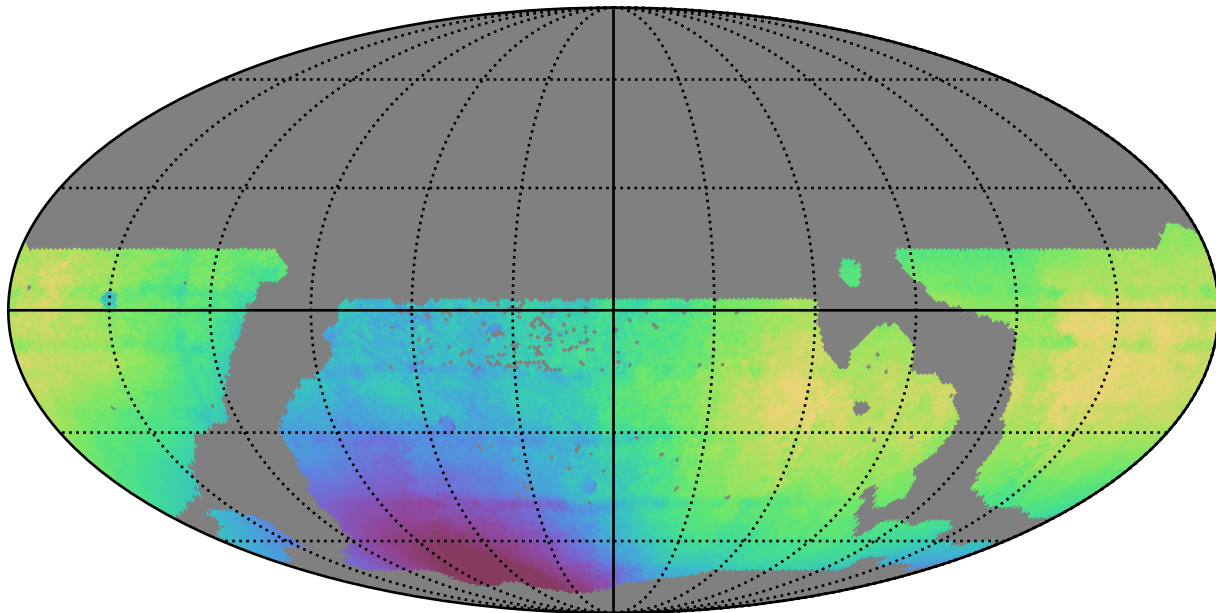
weather_cloudso30v3.4_10yrs WFD all bands: Median solarElong
