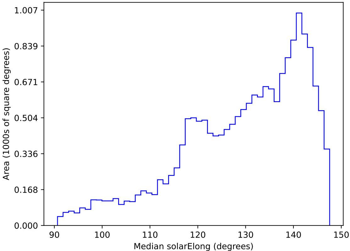
weather_cloudso30v3.4_10yrs WFD all bands: Median solarElong
