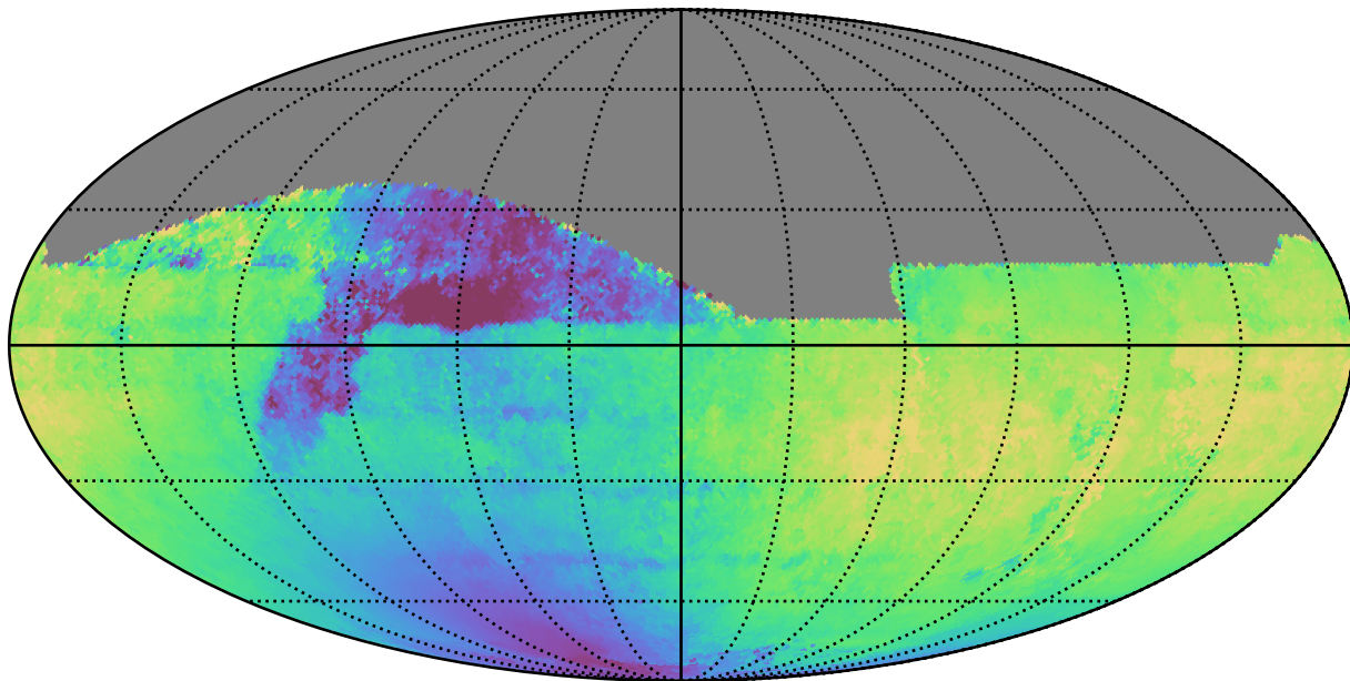
weather_cloudso30v3.4_10yrs All sky z band: Median solarElong
