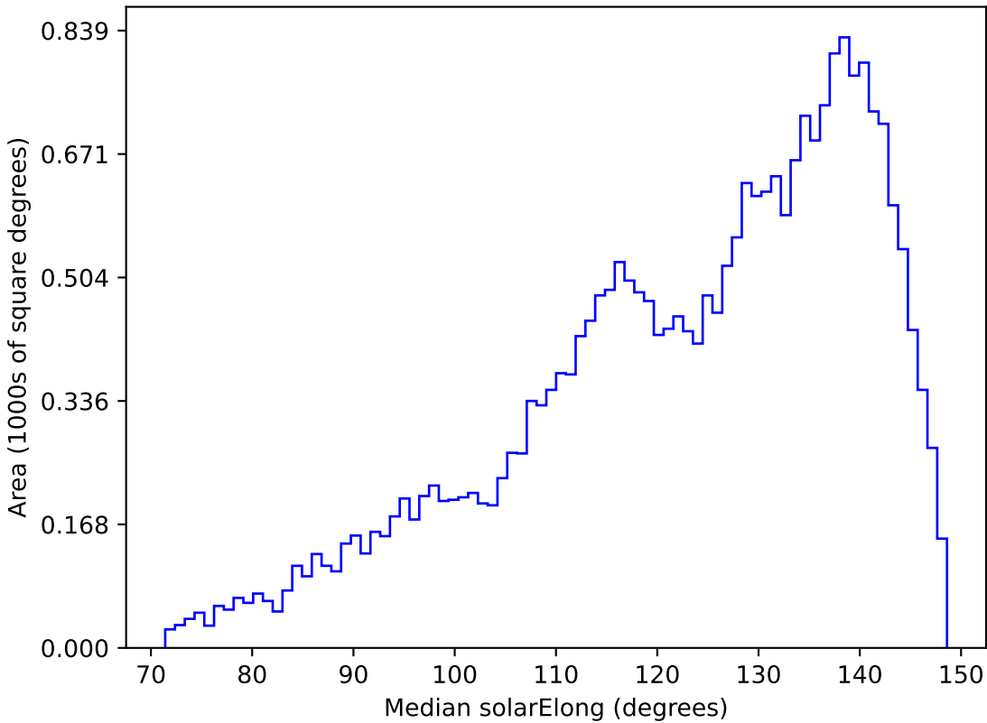
weather_cloudso30v3.4_10yrs All sky z band: Median solarElong
