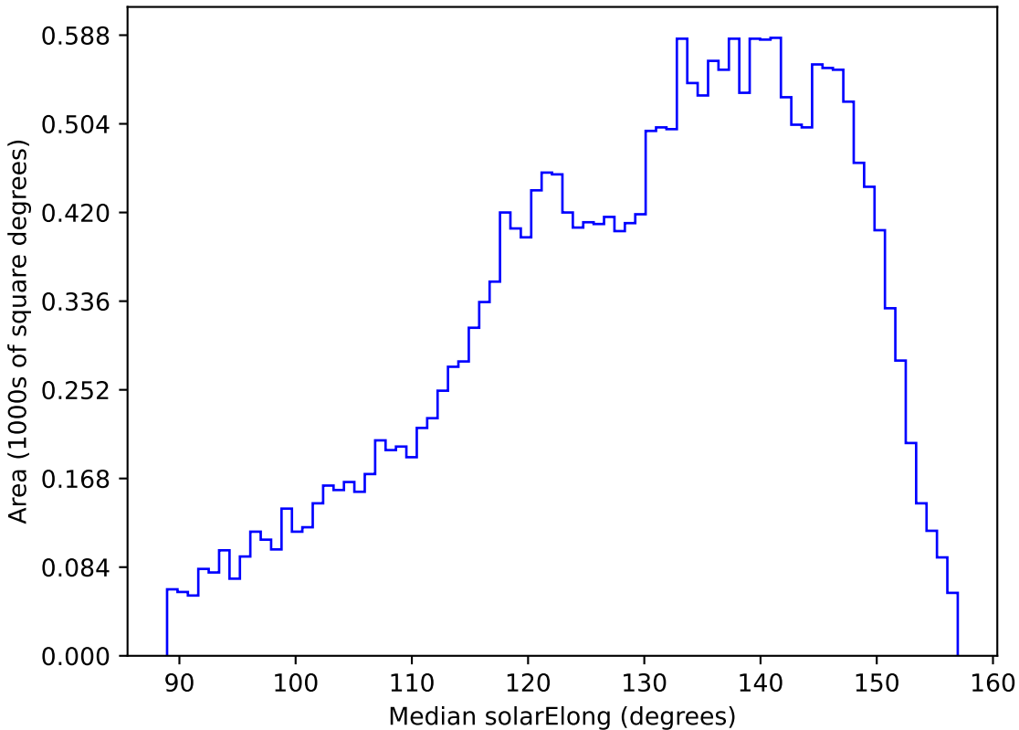
weather_cloudso30v3.4_10yrs All sky u band: Median solarElong
